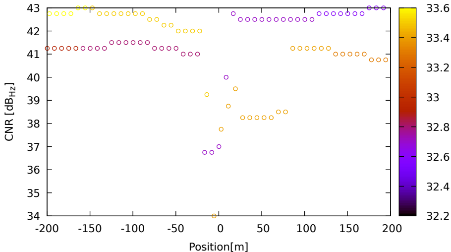
CNR vs position for G22 (L1) on Xiaomi11T - DOY 263 jam. 3
