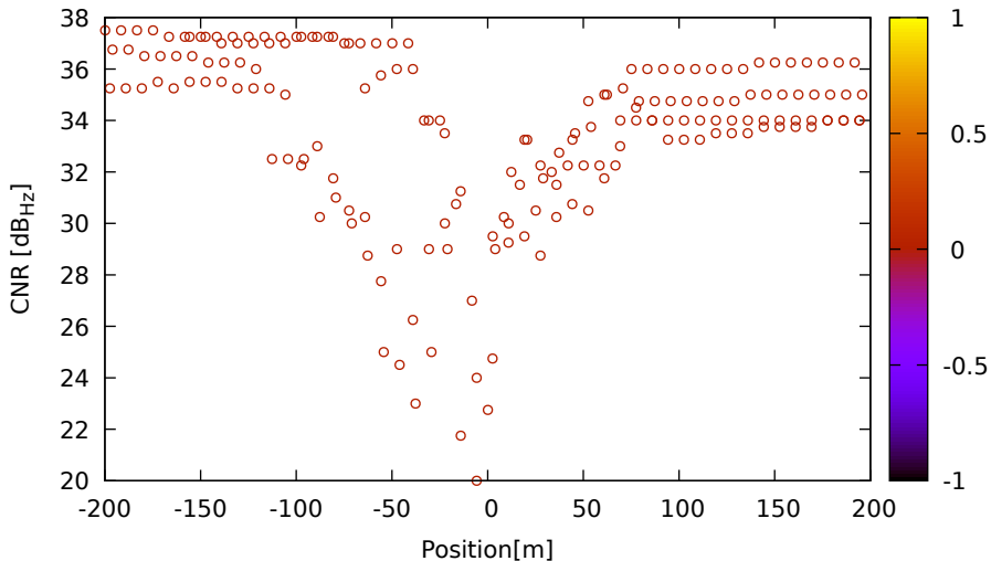
CNR vs position for G28 (L1) on Xiaomi11T - DOY 263 jam. 2
