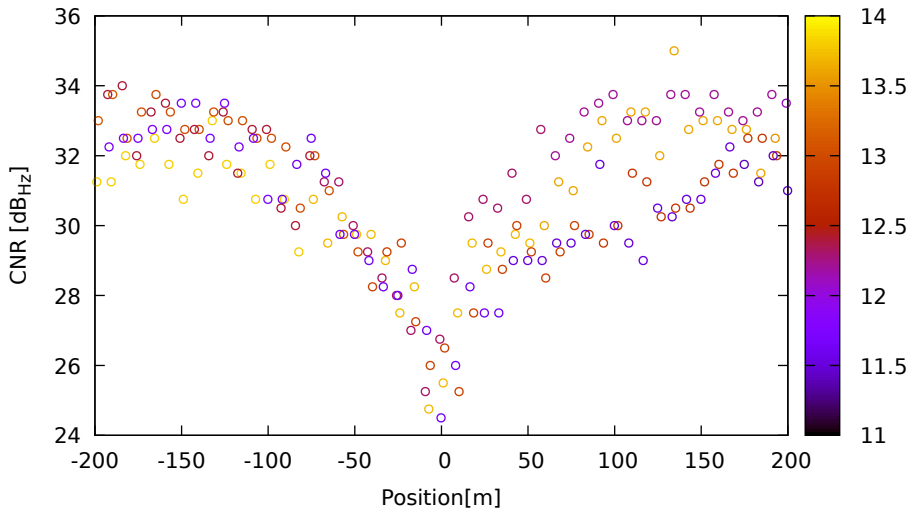
CNR vs position for G32 (L5) on Xiaomi11T - DOY 263 jam. 1
