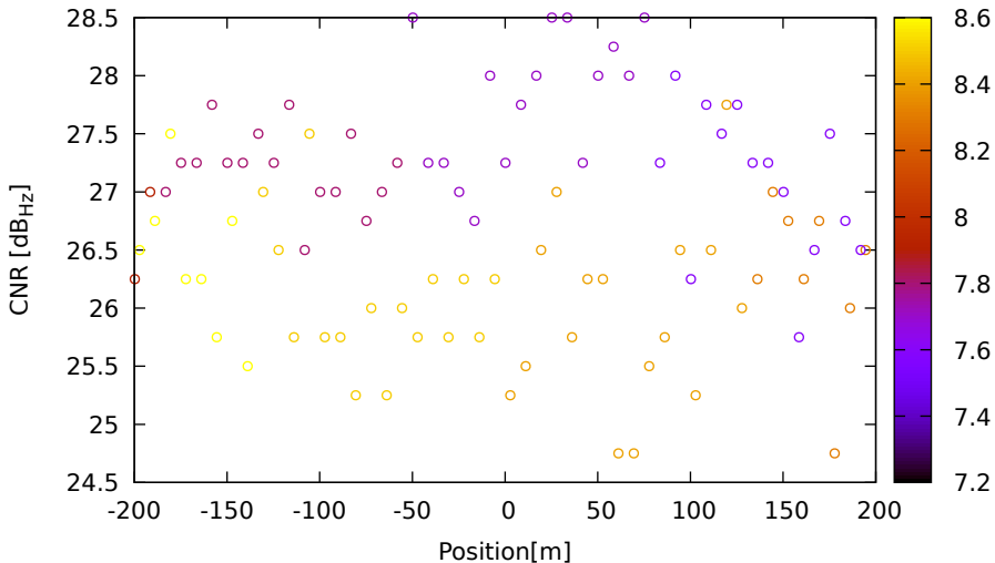
CNR vs position for G32 (L5) on Xiaomi11T - DOY 263 jam. 3
