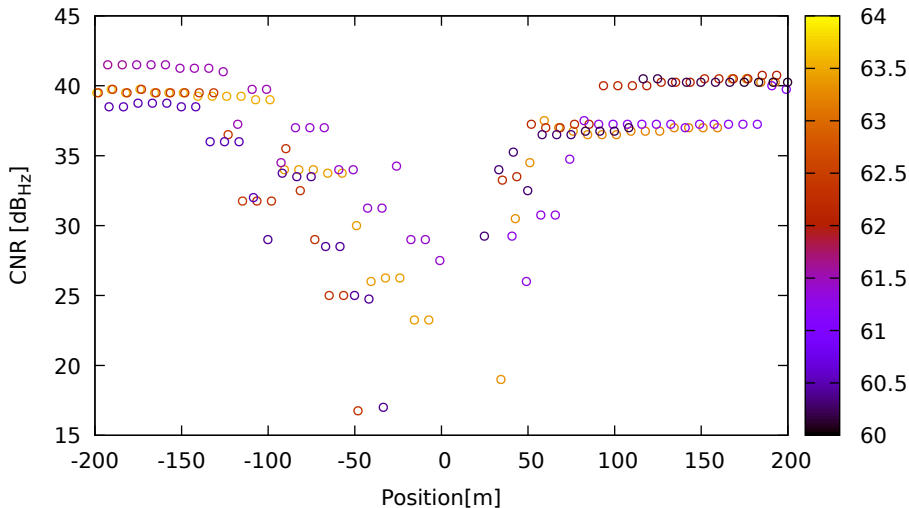
CNR vs position for R01 (G1) on Xiaomi11T - DOY 263 jam. 1
