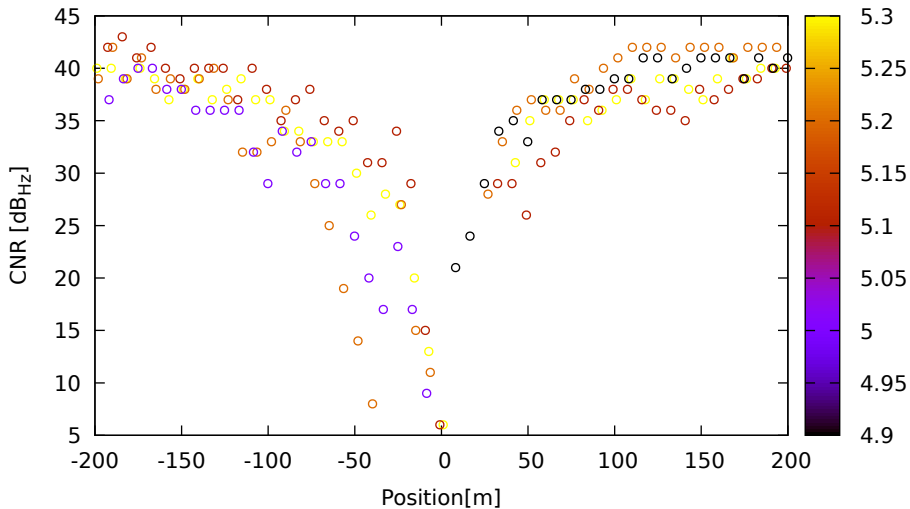
CNR vs position for R09 (G1) on Xiaomi11T - DOY 263 jam. 1
