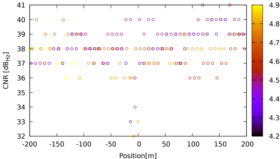
CNR vs position for R09 (G1) on Xiaomi11T - DOY 263 jam. 2
