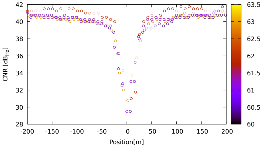
CNR vs position for C11 (B1) on XiaomiMi8 - DOY 263 jam. 1
