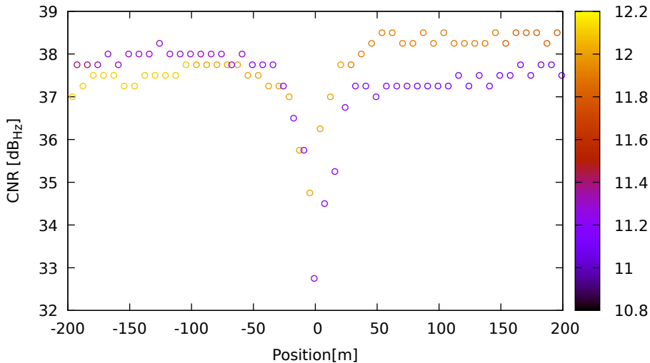
CNR vs position for C12 (B1) on XiaomiMi8 - DOY 263 jam. 3
