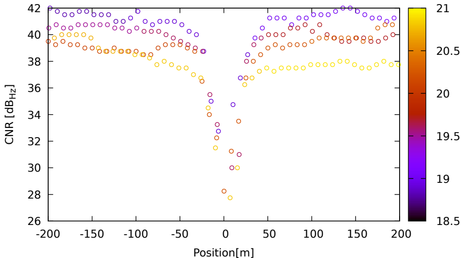
CNR vs position for C28 (B1) on XiaomiMi8 - DOY 263 jam. 1
