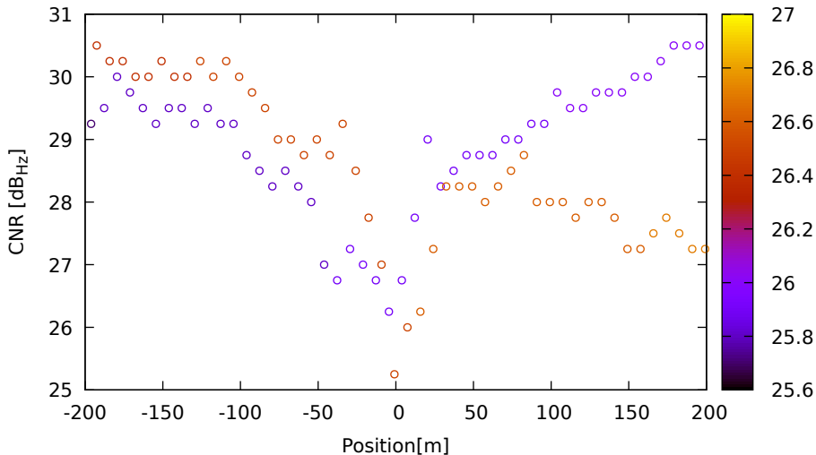
CNR vs position for C33 (B1) on XiaomiMi8 - DOY 263 jam. 3
