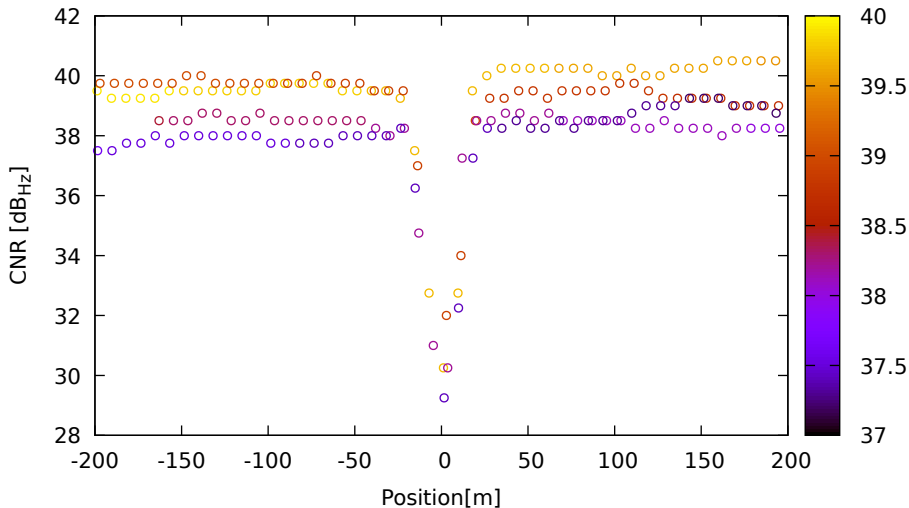
CNR vs position for C34 (B1) on XiaomiMi8 - DOY 263 jam. 2
