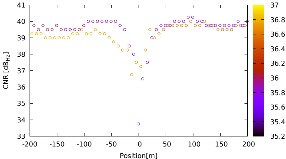
CNR vs position for C34 (B1) on XiaomiMi8 - DOY 263 jam. 3
