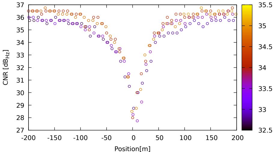
CNR vs position for E04 (E1) on XiaomiMi8 - DOY 263 jam. 1
