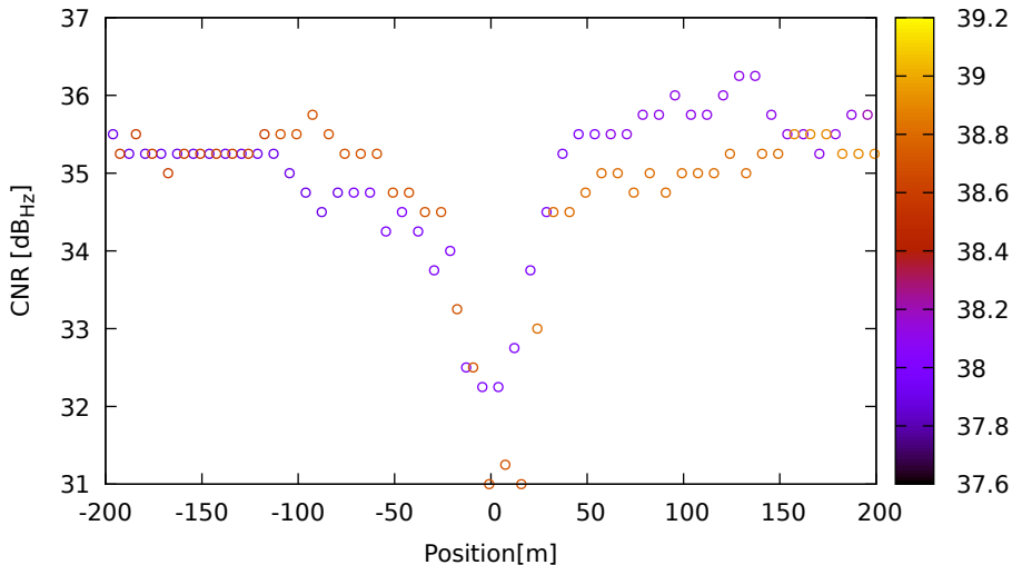
CNR vs position for E04 (E1) on XiaomiMi8 - DOY 263 jam. 3
