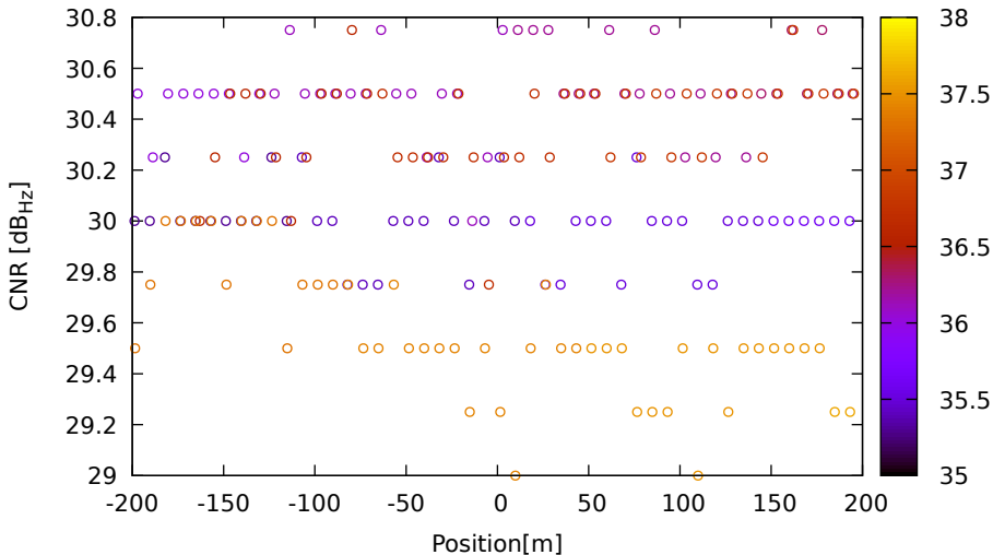
CNR vs position for E04 (E5a) on XiaomiMi8 - DOY 263 jam. 2
