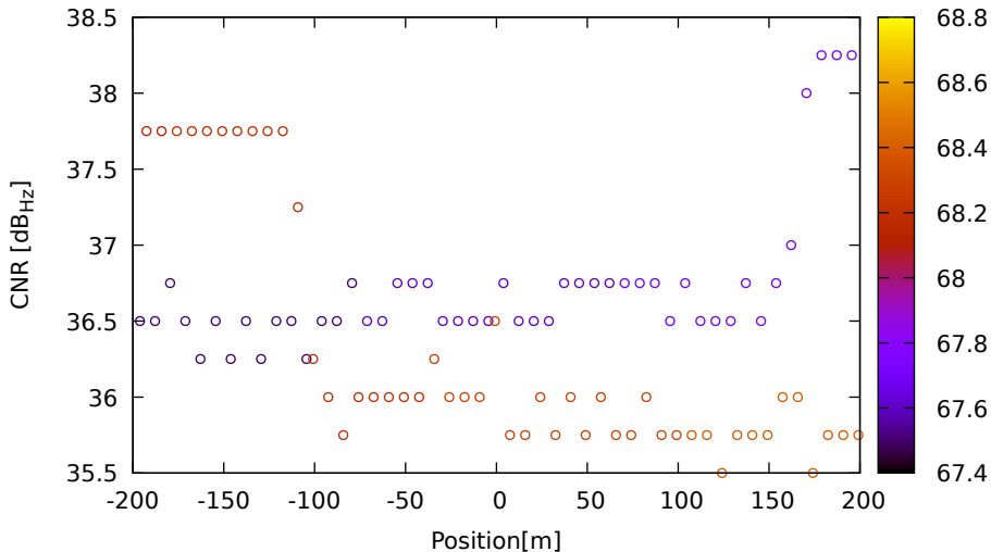
CNR vs position for E10 (E5a) on XiaomiMi8 - DOY 263 jam. 3
