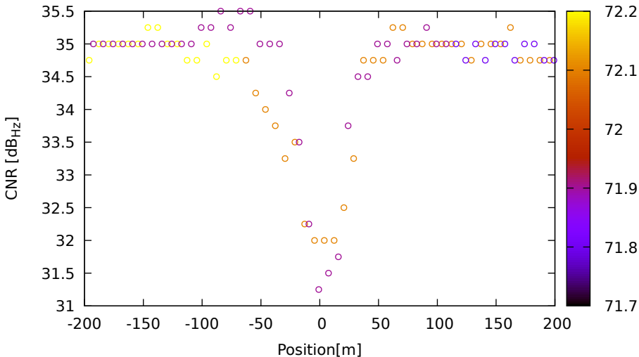
CNR vs position for E19 (E1) on XiaomiMi8 - DOY 263 jam. 3
