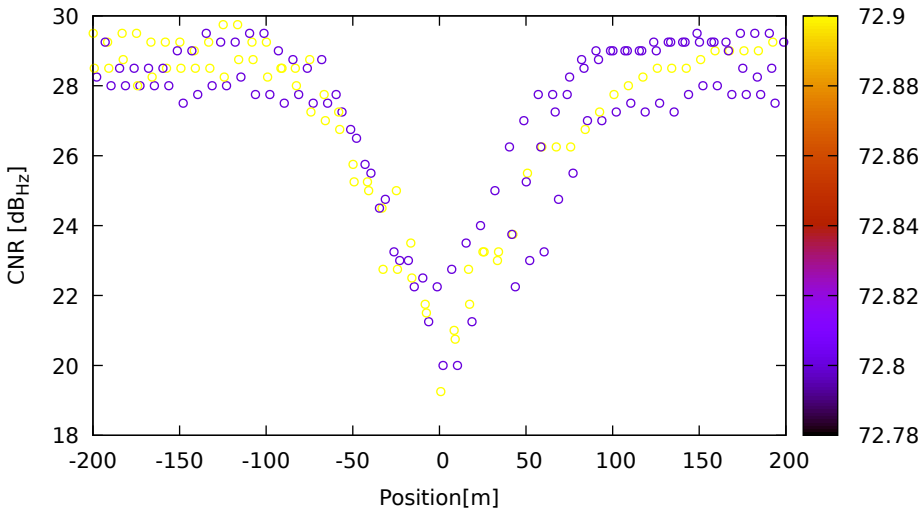
CNR vs position for E19 (E5a) on XiaomiMi8 - DOY 263 jam. 1
