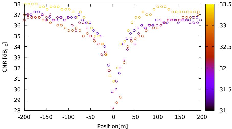
CNR vs position for E33 (E1) on XiaomiMi8 - DOY 263 jam. 1
