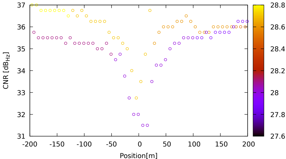
CNR vs position for E33 (E1) on XiaomiMi8 - DOY 263 jam. 3
