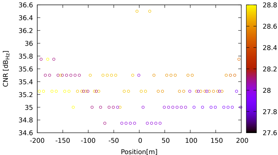
CNR vs position for E33 (E5a) on XiaomiMi8 - DOY 263 jam. 3
