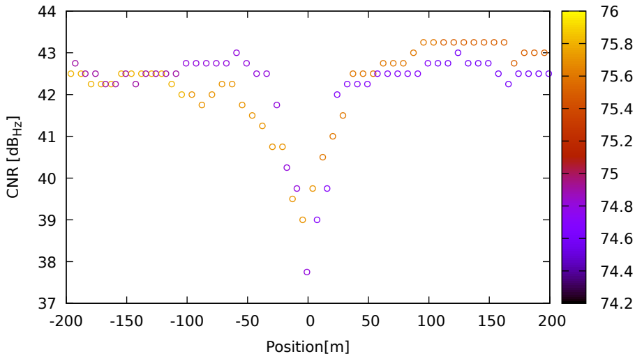
CNR vs position for G01 (L1) on XiaomiMi8 - DOY 263 jam. 3
