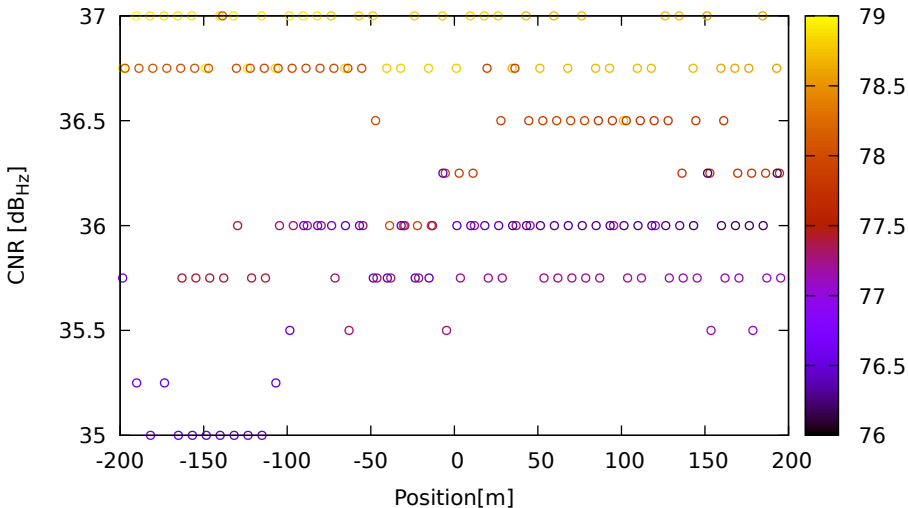
CNR vs position for G01 (L5) on XiaomiMi8 - DOY 263 jam. 2
