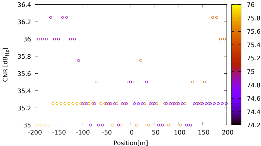
CNR vs position for G01 (L5) on XiaomiMi8 - DOY 263 jam. 3
