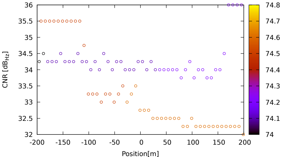
CNR vs position for G03 (L5) on XiaomiMi8 - DOY 263 jam. 3
