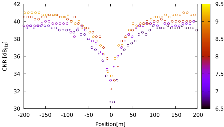
CNR vs position for G08 (L1) on XiaomiMi8 - DOY 263 jam. 1
