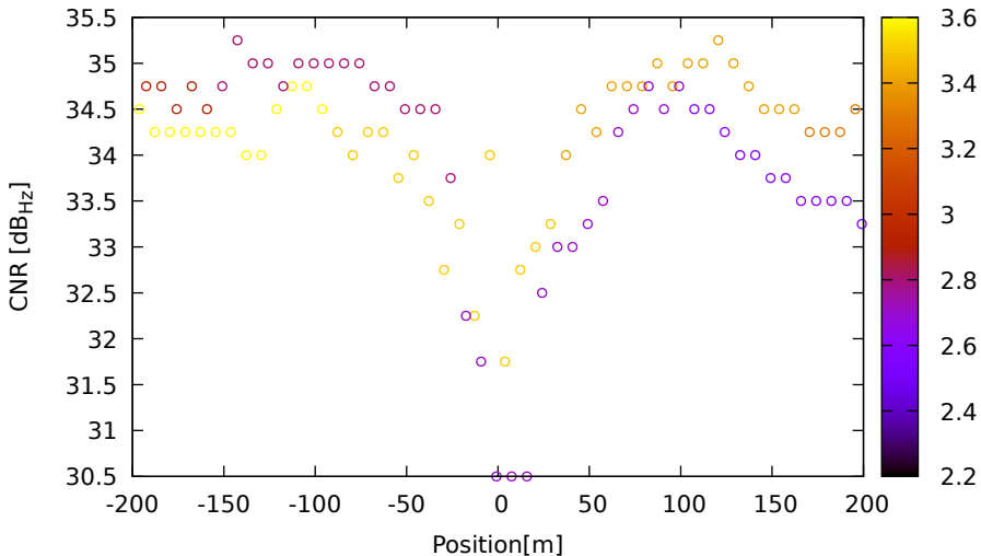
CNR vs position for G08 (L1) on XiaomiMi8 - DOY 263 jam. 3
