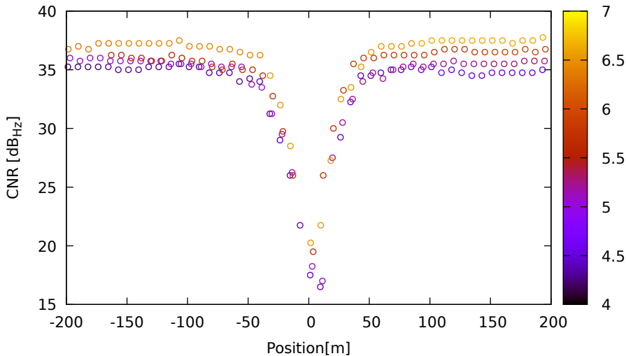
CNR vs position for G09 (L1) on XiaomiMi8 - DOY 263 jam. 2
