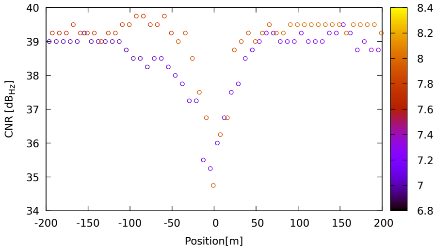
CNR vs position for G09 (L1) on XiaomiMi8 - DOY 263 jam. 3
