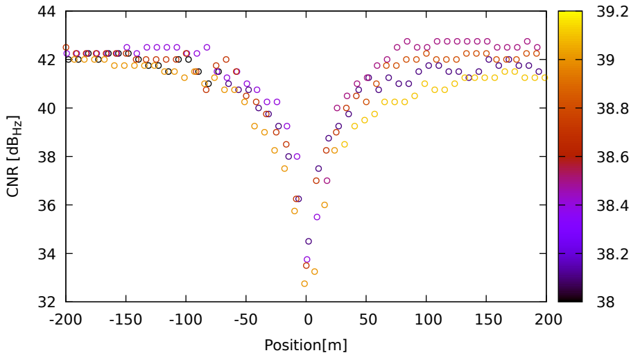
CNR vs position for G17 (L1) on XiaomiMi8 - DOY 263 jam. 1
