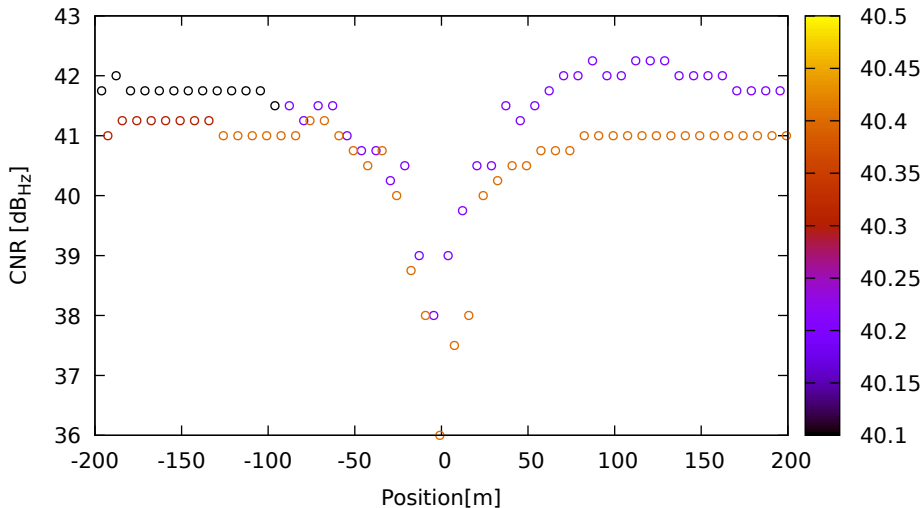
CNR vs position for G17 (L1) on XiaomiMi8 - DOY 263 jam. 3
