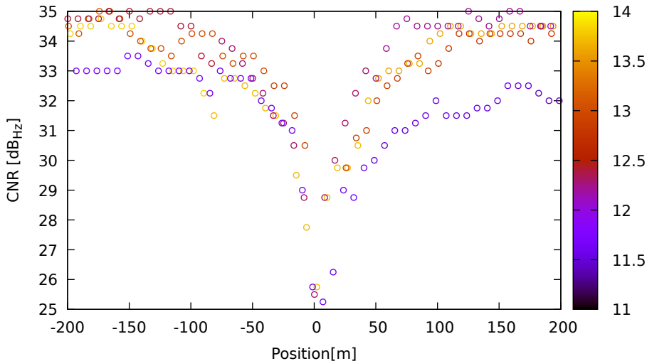
CNR vs position for G32 (L1) on XiaomiMi8 - DOY 263 jam. 1
