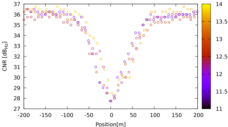
CNR vs position for G32 (L5) on XiaomiMi8 - DOY 263 jam. 1
