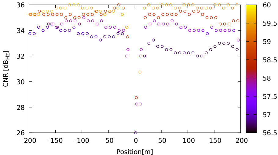
CNR vs position for R01 (G1) on XiaomiMi8 - DOY 263 jam. 2
