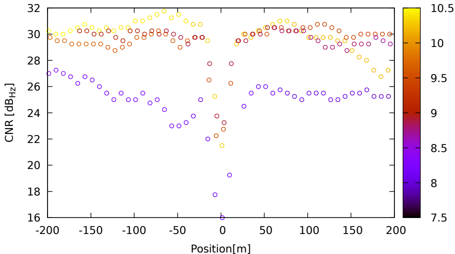
CNR vs position for R08 (G1) on XiaomiMi8 - DOY 263 jam. 2
