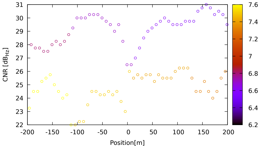
CNR vs position for R08 (G1) on XiaomiMi8 - DOY 263 jam. 3
