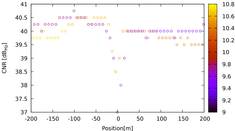
CNR vs position for R23 (G1) on XiaomiMi8 - DOY 263 jam. 3
