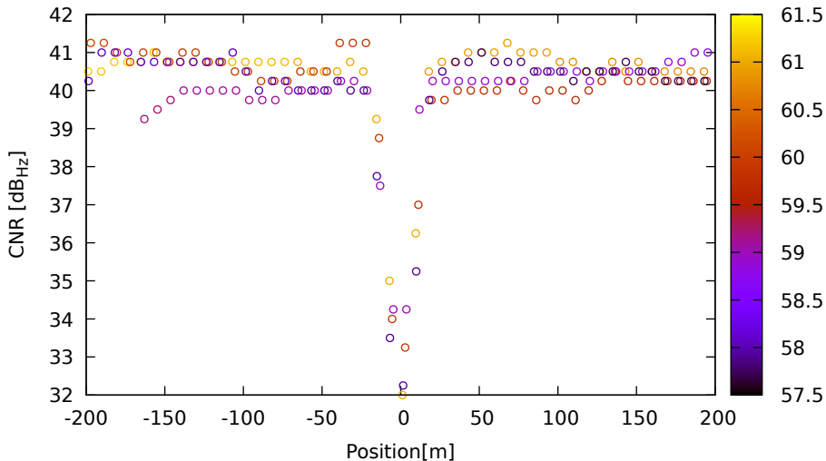
CNR vs position for R24 (G1) on XiaomiMi8 - DOY 263 jam. 2
