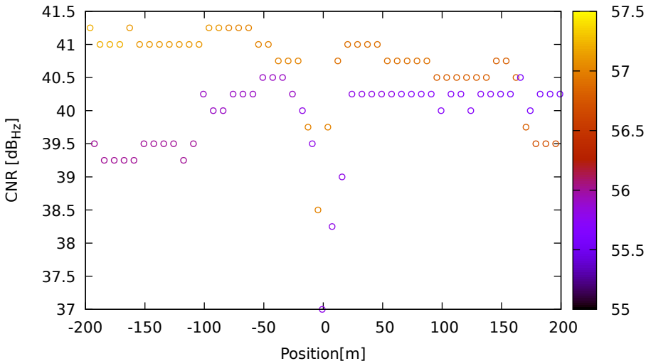
CNR vs position for R24 (G1) on XiaomiMi8 - DOY 263 jam. 3
