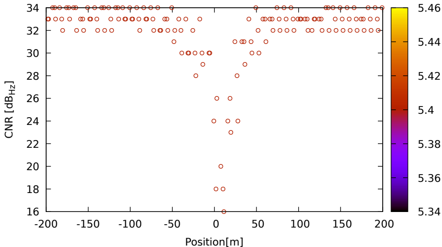
CNR vs position for C02 (B1) on HuaweiP40 - DOY 263 jam. 1
