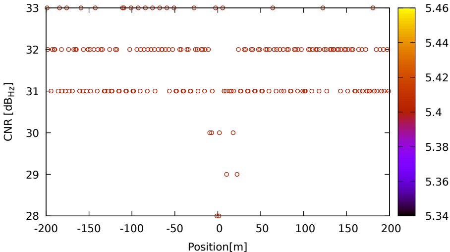
CNR vs position for C02 (B1) on HuaweiP40 - DOY 263 jam. 2
