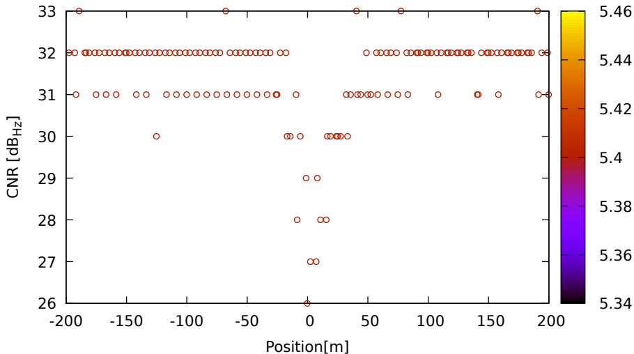
CNR vs position for C02 (B1) on HuaweiP40 - DOY 263 jam. 3
