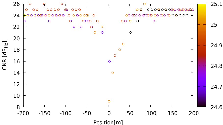
CNR vs position for C06 (B1) on HuaweiP40 - DOY 263 jam. 1
