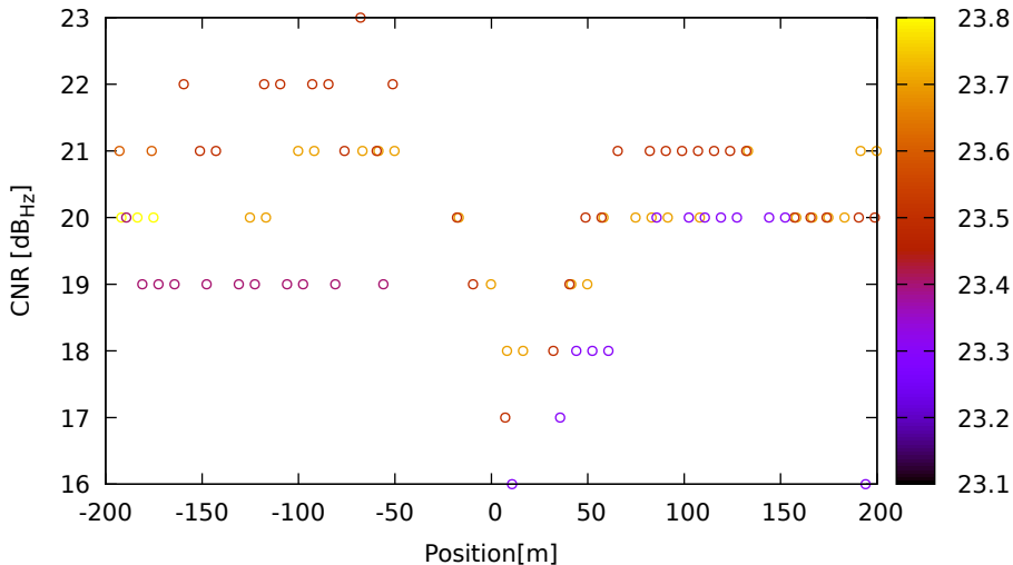
CNR vs position for C06 (B1) on HuaweiP40 - DOY 263 jam. 3
