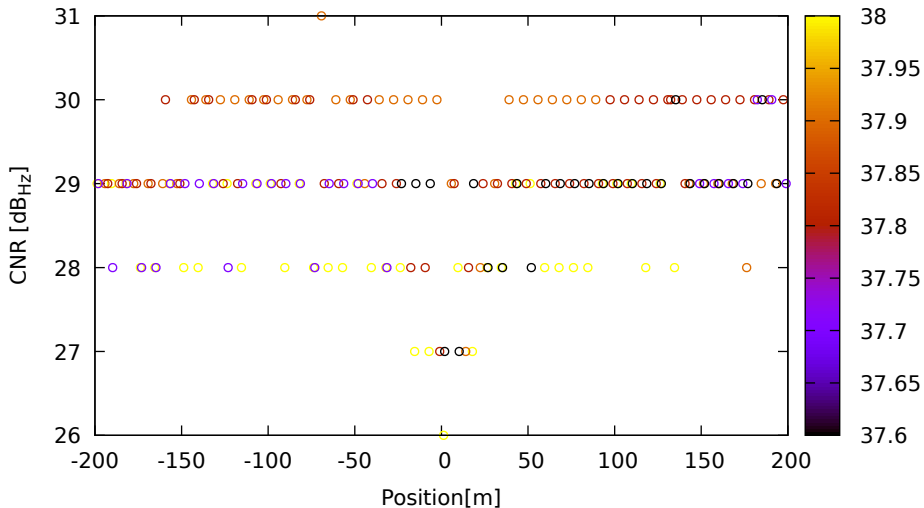
CNR vs position for C09 (B1) on HuaweiP40 - DOY 263 jam. 2
