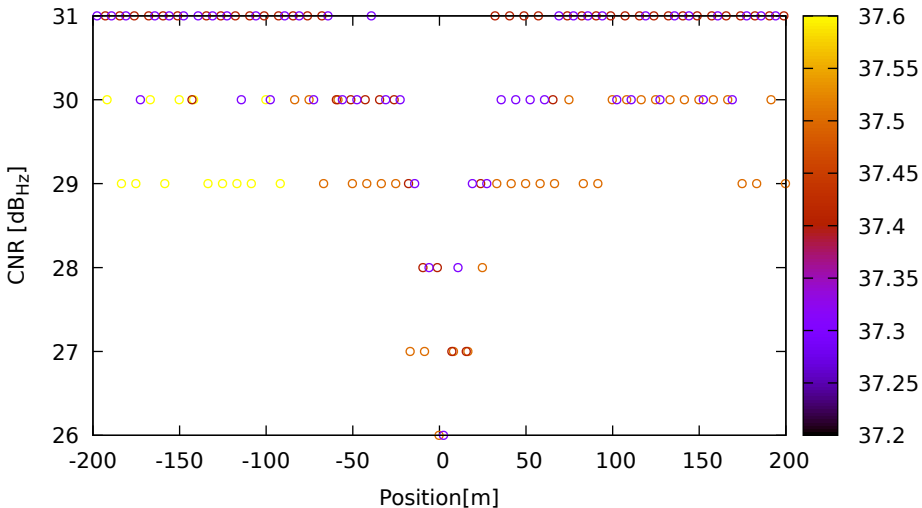
CNR vs position for C09 (B1) on HuaweiP40 - DOY 263 jam. 3
