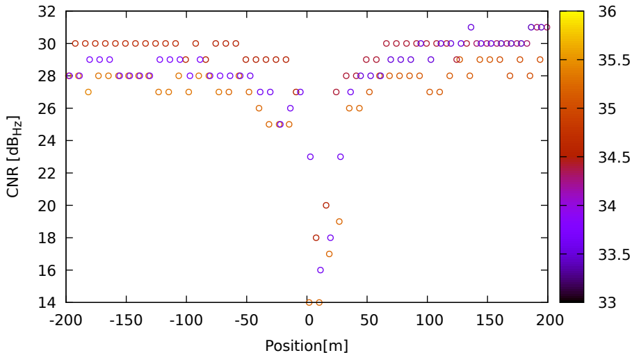
CNR vs position for C11 (B1) on HuaweiP40 - DOY 263 jam. 1
