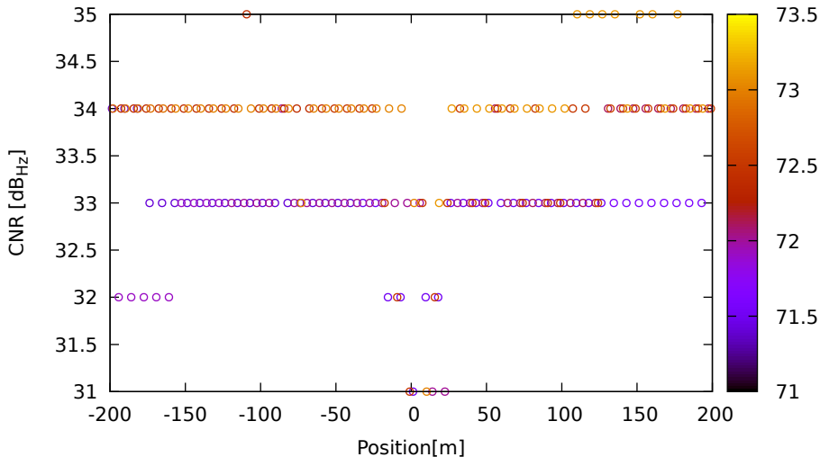
CNR vs position for C14 (B1) on HuaweiP40 - DOY 263 jam. 2
