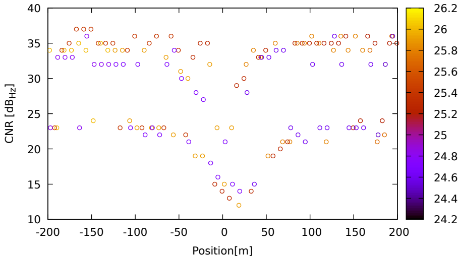
CNR vs position for C21 (B1) on HuaweiP40 - DOY 263 jam. 1
